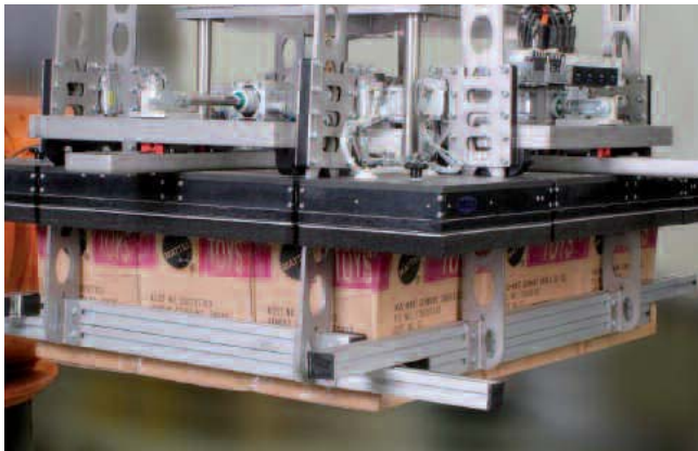
Large-area vacuum gripping system SPZ with flexible foam and auxiliary mechanical gripper for handling complete layers of cardboard boxes
