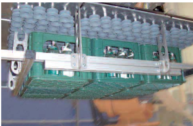
Large-area vacuum gripping system SPZ with individual suction pads and auxiliary mechanical gripper for handling crates of mineral water
