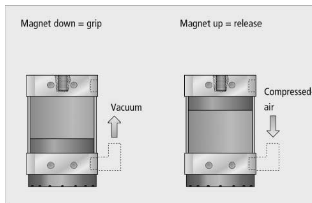
Operation with compact ejector
